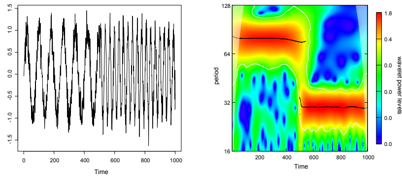
Figure 10. The original sinusoidal signal with two periods, P = 80 for the first part of the curve and P = 30 for the final part is shown on the left panel. The corresponding scalogram with the evidence of the two detected periods and the time interval involving each one is shown on the right panel.
